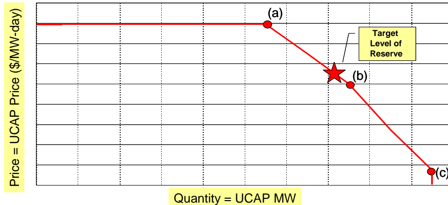
Exhibit 14: Illustrative Example of a Variable Resource Requirement Curve
