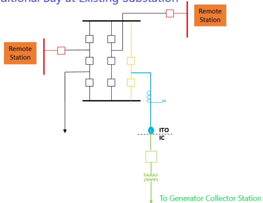
Additional Bay at Existing Substation
