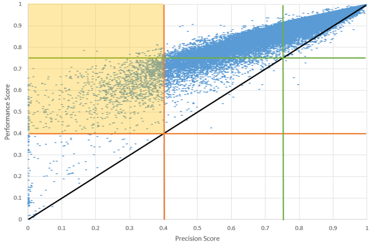
Performance Score vs Precision Score for each Unit-Hour
