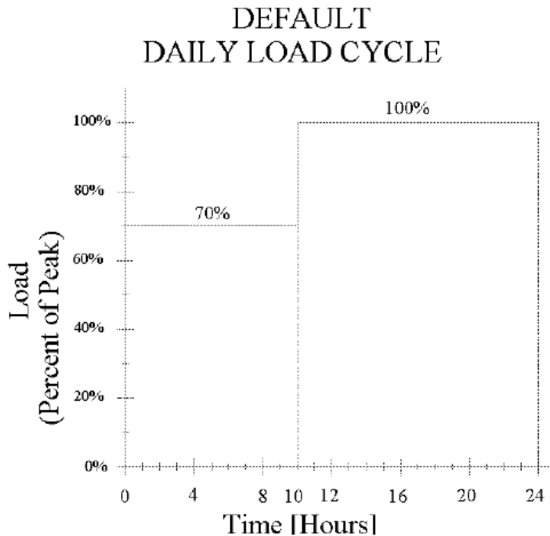
FIGURE 1 Default Load Curve for Normal or Long Time Ratings
