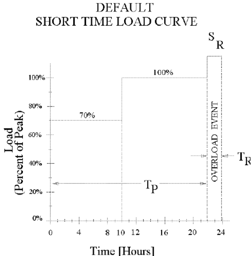
FIGURE 2 Default Load Curve for Emergency Ratings
